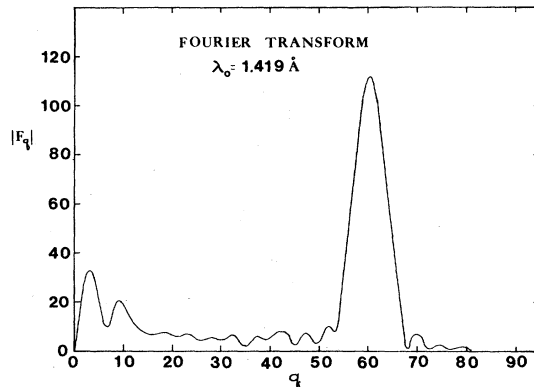
FIG. 14. Fourier transform of the data of Fig. 12.
