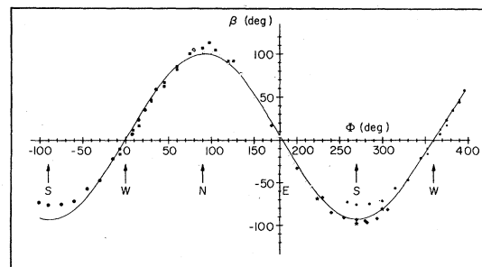
FIG. 21. A plot of the phase shift \beta due to the Earth's rotation as a function of orientation \phi of the normal area \vec{A} of the interferometer about a vertical axis. The symbols N, W, S, and E indicate north, west, south, and east. These data were taken in six sections as discussed in the text. The different symbols are for the interferometer box facing various directions.
