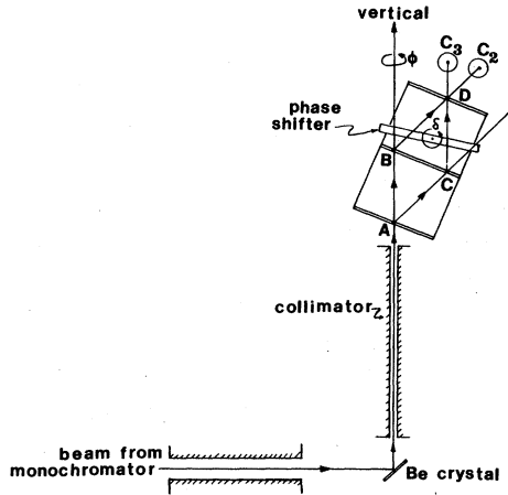
FIG. 18. Schematic diagram of the configuration of the apparatus for the vertical-beam experiments designed to measure the neutron Sagnac effect. The drawing is not to scale. The collimator is approximately 1 m in length, and the interferometer is approximately 8 cm long from point A to point D. The angle \delta of the phase shifter is defined to be zero when it is parallel to the three interferometer slabs.
