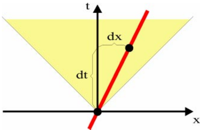
Fig. 2. (Color online) A spacetime diagram showing the worldline of the moving clock (the fat line). The two events we are considering are the black dots in the diagram. The shaded area is known as the lightcone.
