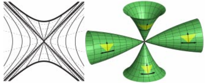
Fig. 16. (Color online) To the left: A Kruskal diagram of a maximally extended black hole. To the right: an embedding of the absolute geometry with generators at fixed radius in the exterior regions and at fixed Schwarzschild time in the interior regions (the full drawn lines in the diagram).
