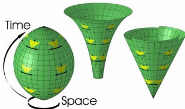
Fig. 6. (Color online) Schematic spacetime cosmological models.
