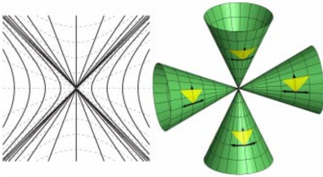
Fig. 15. (Color online) To the left: Minkowski spacetime with a certain set (as discussed in the main text) of worldlines (the thick full drawn lines). To the right: The corresponding absolute geometry embedding. Note that the conical surfaces are not closed as one goes around in the space direction, but rather they consist of very tightly rolled layers with no end.
