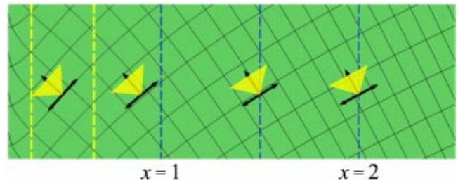
Fig. 13. (Color online) A flat embedding of a Reissner–Nordström black hole. The dimensionless radial coordinate x lies in the range [0.22, 2.5] . The two internal horizons are marked with the thicker dotted lines. The charge is chosen so that \beta=0.95 .
