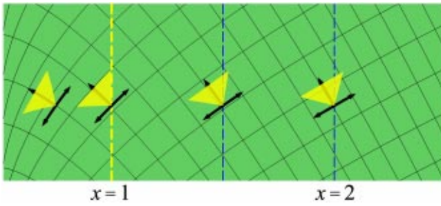
Fig. 12. (Color online) A flat embedding of a Schwarzschild black hole. The radial parameter x lies in the interval [0.5, 2.5] . We could equivalently embed this geometry as a cylinder. As we go further to the right (larger x ), the lightcones will approach pointing straight up.
