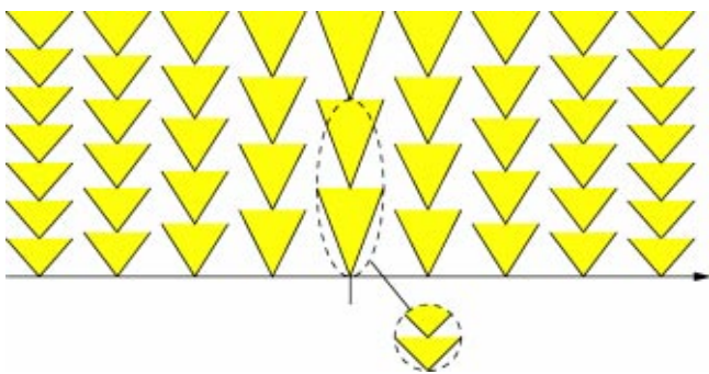
Fig. 18. (Color online) A flat spacetime visualization of a radial line through a star. The lightcones are everywhere, by definition, one proper time unit high, and two proper length units wide. The dashed circle illustrates that when we actually go to a specific region, the lightcones will appear as they do at infinity.
