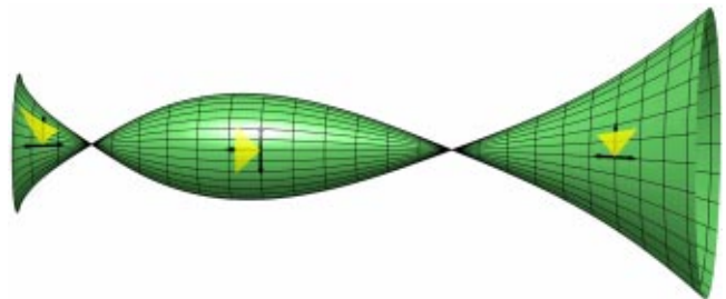
Fig. 14. (Color online) An alternative representation of a Reissner–Nordström black hole. Notice the direction of the local Minkowski systems. Here \beta=0.995 and the range is [0.425, 0.7] .
