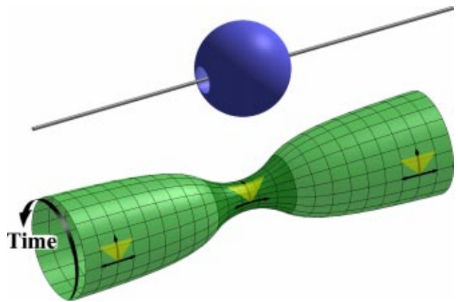
Fig. 4. (Color online) A radial line through a very dense star, and an illustration of the curved spacetime for that line. Time is directed around the hourglass-shaped surface. Strictly speaking the surface should not close in on itself in the time direction. Rather one should come to a new layer after one circumference as on a paper roll.
