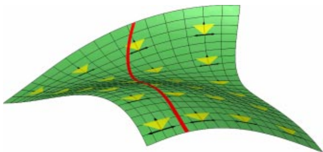
Fig. 3. (Color online) An illustration of curved spacetime using a curved surface with little Minkowski systems living on it. The curving line could be the worldline of a moving clock.
