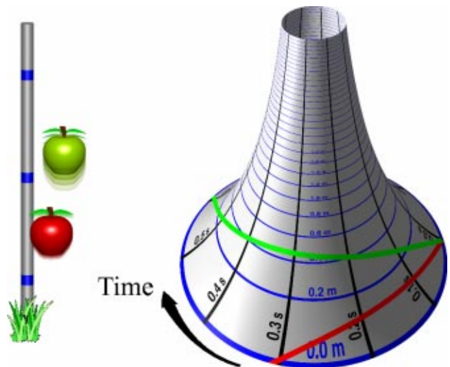
Fig. 19. (Color online) Illustration of how straight lines in a curved spacetime can explain the motion of upwards-thrown apples. The lines can be found using a little toy car that is rolled straight ahead on the surface.
