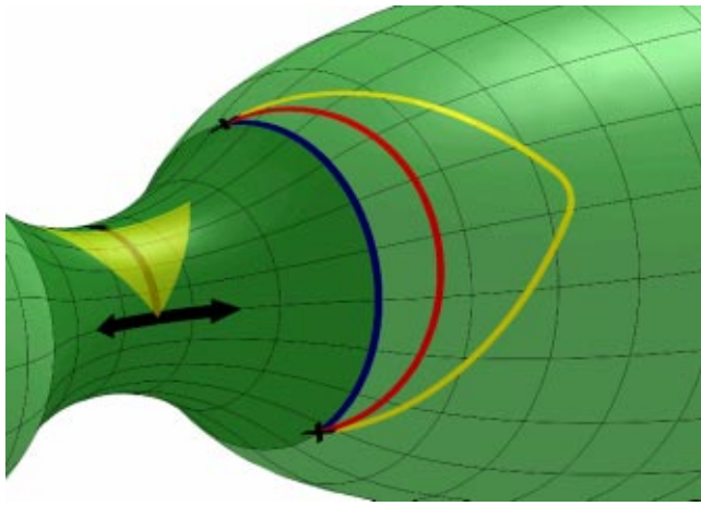
Fig. 5. (Color online) Three different worldlines connecting two fixed events. The middle worldline corresponds to the actual motion of an object initially thrown radially away from the star and then falling back toward the star. Of the three worldlines this has the largest integrated proper time.
