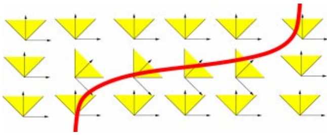
Fig. 17. (Color online) A crude illustration of a toy model for warp drive.
