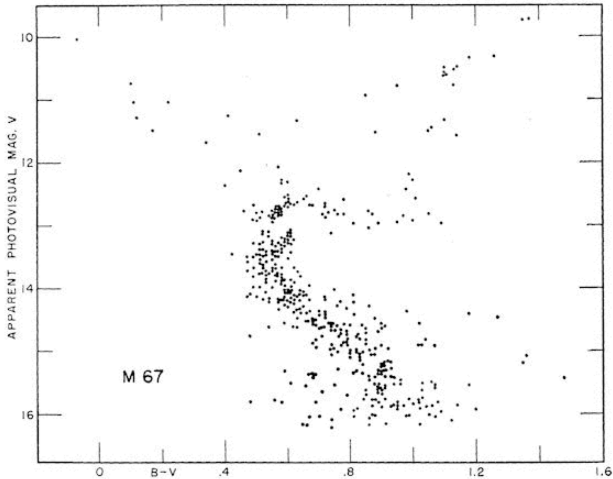
FIG. 3.—The color-magnitude diagram for M67
