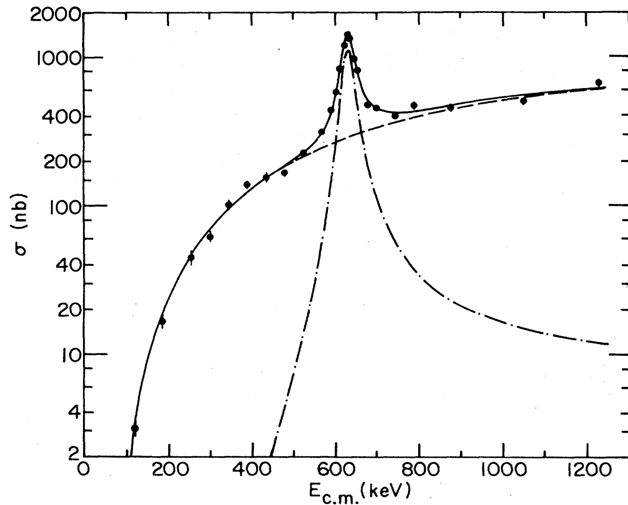
Cross Section \sigma(E)
