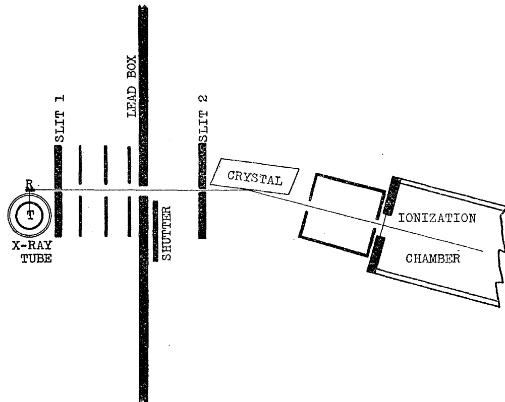
Fig. 1. Measuring the wave-length of scattered x-rays.
