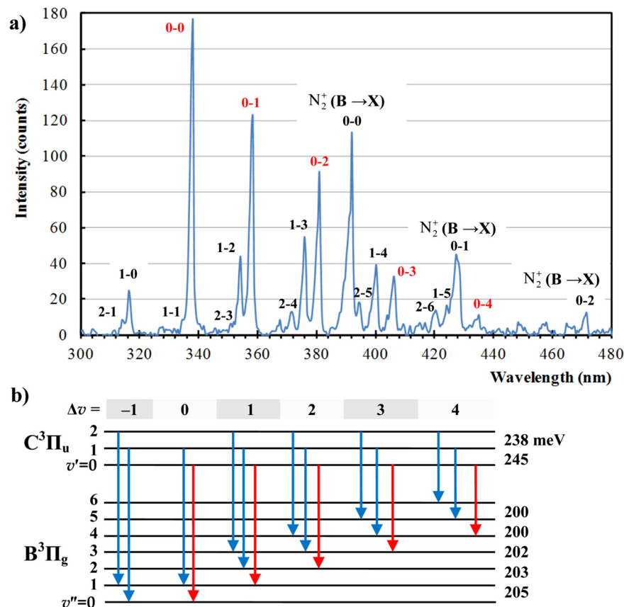
Fig. 2. (Color online) (a) A typical emission spectrum from the discharge tube, exhibiting both \text{N}_2(C^3\Pi \rightarrow B^3\Pi) and \text{N}_2^+(B^2\Sigma \rightarrow X^2\Sigma) radiative decays, with assigned vibrational quantum numbers v' - v'' . (b) Vibrational energy level diagram for the \text{N}_2 transitions represented by the shown spectrum. The transition arrows are arranged in sequences of constant \Delta v , vertically aligned with the respective spectral bands.
