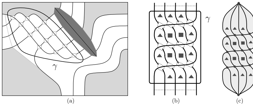
FIGURE 5. (a) Decompose M(n, m, r, s) into tetrahedra, here r = 5 , s = 3 and \beta = \bar{\delta}_5 . Thick lines are link components, dotted lines are polygon edges. This figure differs from Figure 4 (middle) only in the encircled region. (b) For \beta = \bar{\delta}_5 , schematic figure for \beta^3 with triangles and quadrilaterals indicated. (c) The disk triangulated with the projection of \beta^3 .
