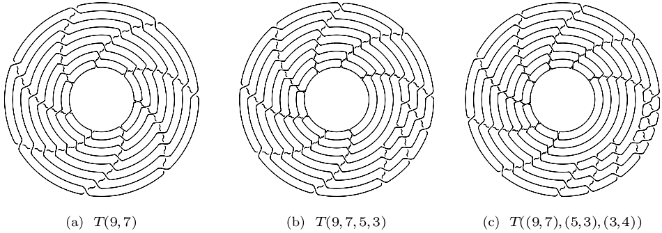
FIGURE 2. A torus knot, a twisted torus knot, and a T -knot using standard roots.
