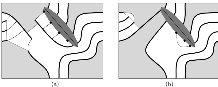
FIGURE 9. After collapsing as in Figure 8, regions on T^2 \times \{0\} seen from the top in (a) and from the bottom in (b).
