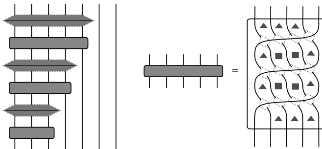
FIGURE 12. Schematic figure of a general T -link, with triangles and quadrilaterals indicated for the root \bar{\delta}_5 .
