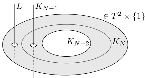
FIGURE 14. The knot K = K_N lives on a four-punctured sphere in M_N .
