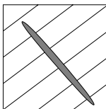
FIGURE 1. The regular neighborhood of a line segment crossing r strands.
