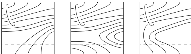
FIGURE 3. M(3, 7, 5, 0) is homeomorphic to M(3, 4, 5, 0) .
