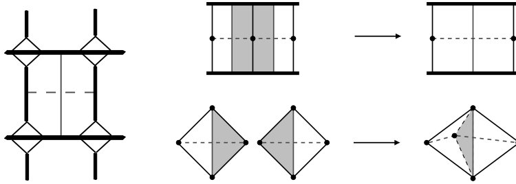
FIGURE 7. Left: medial tetrahedron inserted at every inner quadrilateral. Right: adjacent medial tetrahedra are glued together when their triangular faces with common edges are collapsed.
