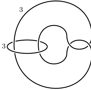
FIGURE 3. The orbifold \mathcal{O}_W , with singular locus the Whitehead link.
