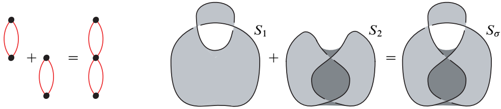
Figure 5: Left: The graph \mathbb{G}_\sigma decomposes as a union of subgraphs \mathbb{G}_1 and \mathbb{G}_2 , joined along the cut vertex v . Right: The corresponding decomposition of S_\sigma as a Murasugi sum of state surfaces S_1 and S_2 .
